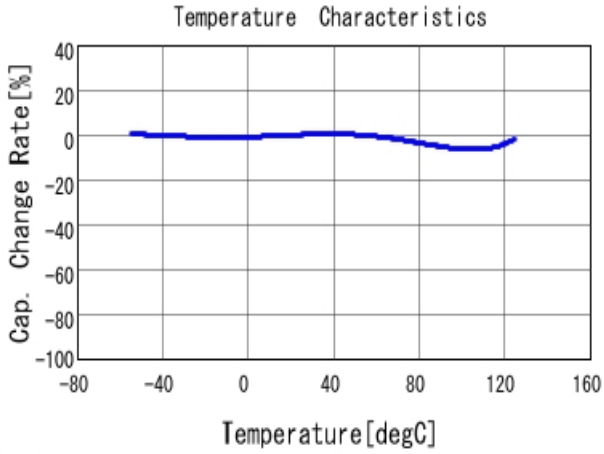
■ GRM155R71H821KA01 C-Temp. capchange, DCO. 0V, AC1.0Vrm
