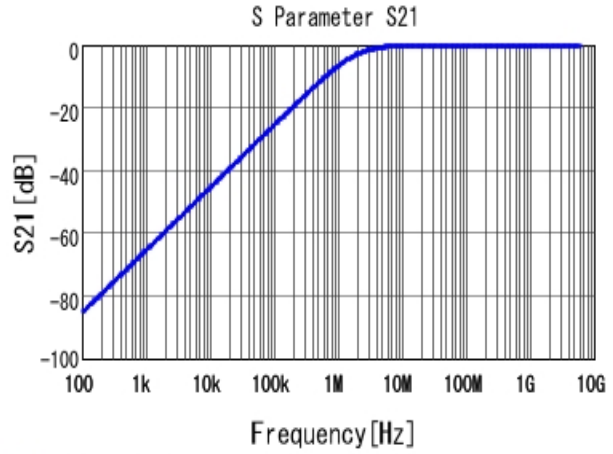
■ GRM155R71H821KA01 S21 DCOV, 25degC
