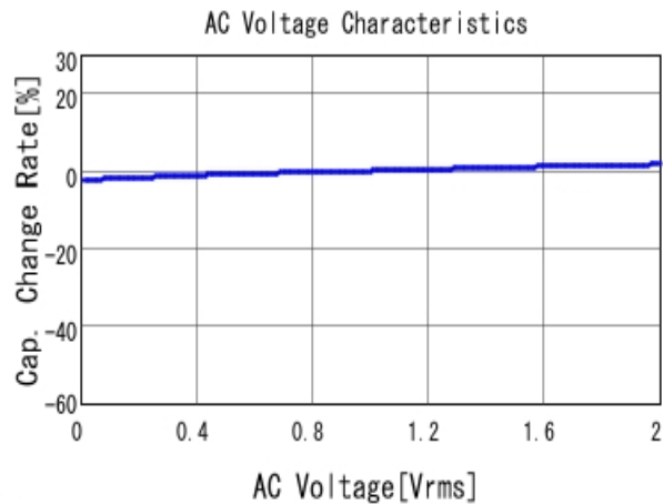
■ GRM155R71H821KA01 C-AC Voltage capchange, DCOV, 25.0d
