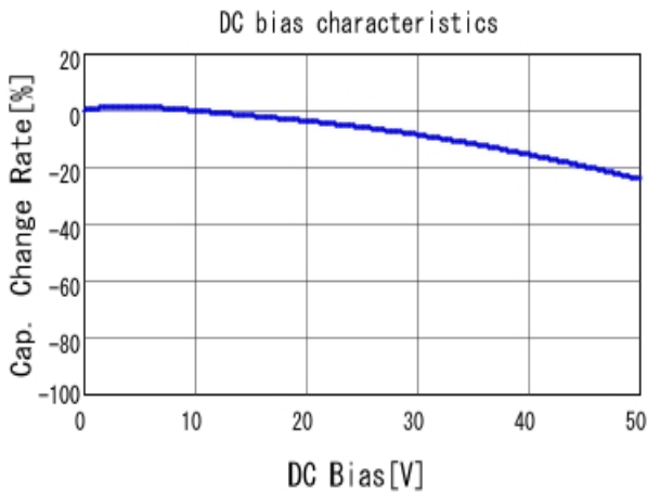
■ GRM155R71H821KA01 C-DC bias capchange, 25.0degC, AC1.
