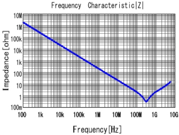
■ GRM155R71H821KA01 |Z| DCOV, 25degC
