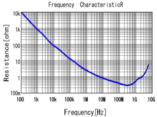
■ GRM155R71H821KA01 R DCOV, 25degC
