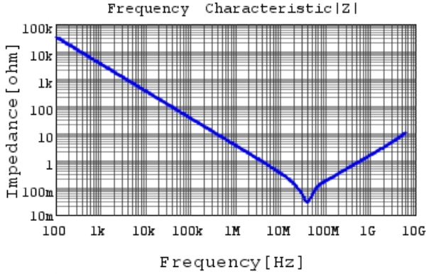
GRM155R71E473JA88 |Z| DCOV, 25degC
