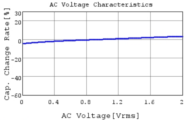
GRM155R71E473JA88 C-AC Voltage capchange, Dc
