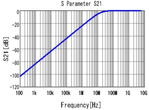
■ GRM033R71C101KA01 S21 DCOV, 25degC
