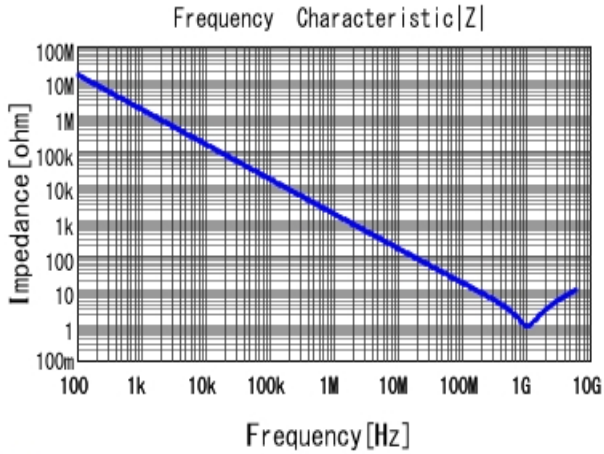
■ GRM033R71C101KA01 |Z| DCOV, 25degC
