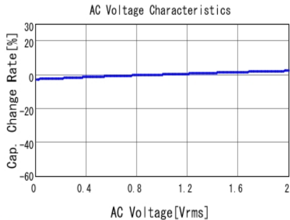
■ GRM033R71C101KA01 C-AC Voltage capchange, DCOV, 25.0d
