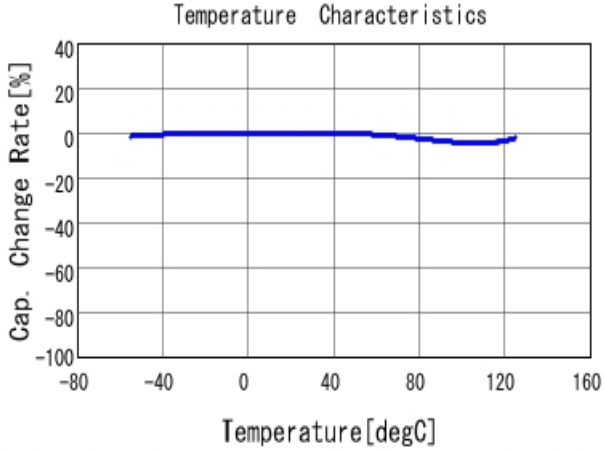
■ GRM033R71C101KA01 C-Temp. capchange, DCO. 0V, AC1.0V rm
