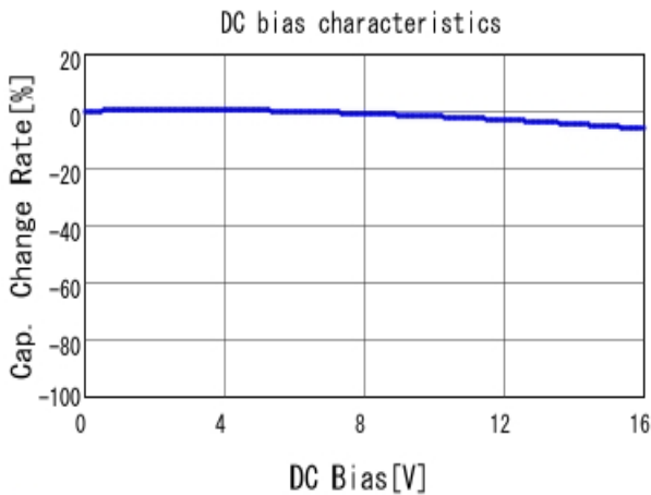
■ GRM033R71C101KA01 C-DC bias capchange, 25.0degC, AC1.
