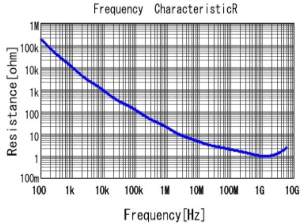
■ GRM033R71C101KA01 R DCOV, 25degC
