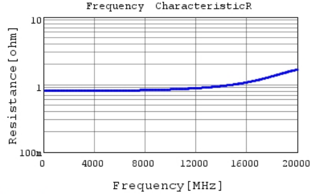
GRM0335C1HR80WA01 R DCOV, 25degC
