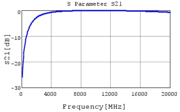
GRM0335C1HR80WA01 S21 DCOV, 25degC
