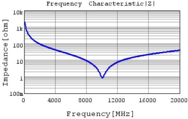
GRM0335C1HR80WA01 |Z| DCOV, 25degC
