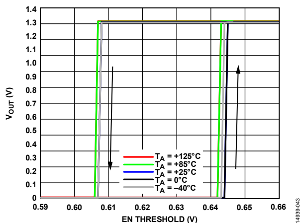
Figure 43. Output Voltage vs. EN Threshold, V_{OUT} = 1.3 V
