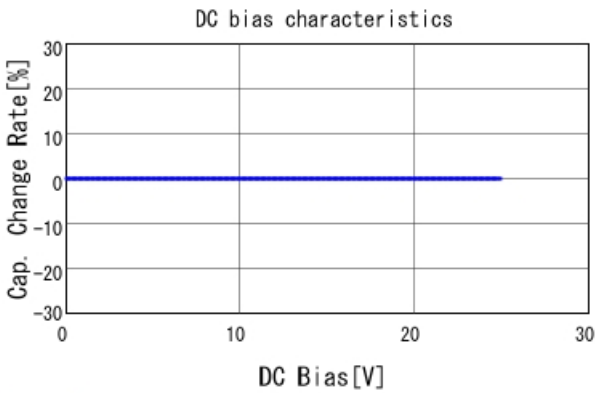
GRM1555C1E561JA01 C-DC bias capchange, 25.0degC, A
