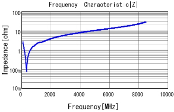
GRM1555C1E561JA01 |Z| DCOV, 25degC
