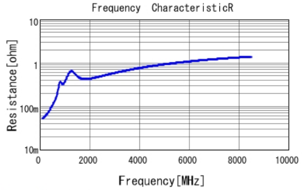
GRM1555C1E561JA01 R DCOV, 25degC
