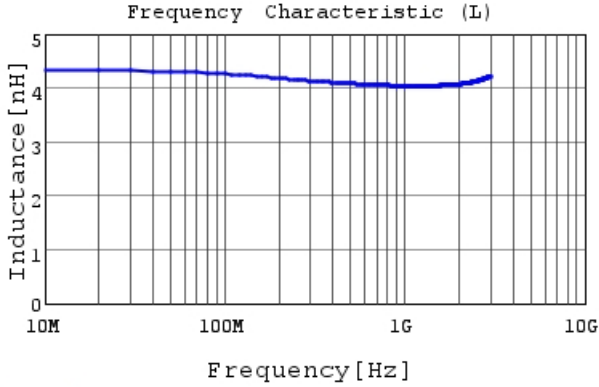
LQP02HQ4N1B02 L
