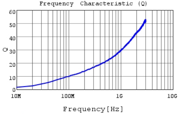
LQP02HQ4N1B02 Q
