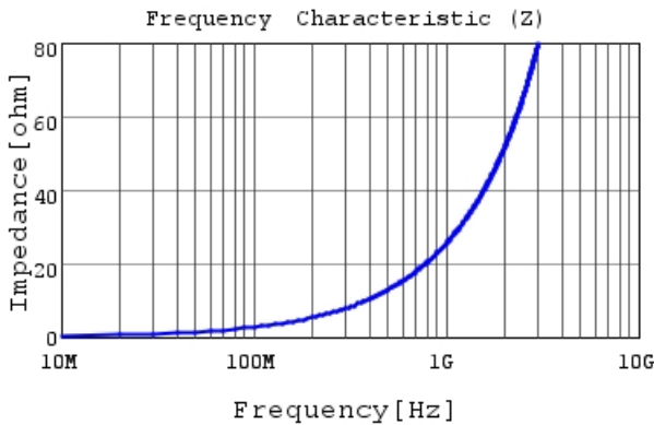
LQP02HQ4N1B02 |Z|
