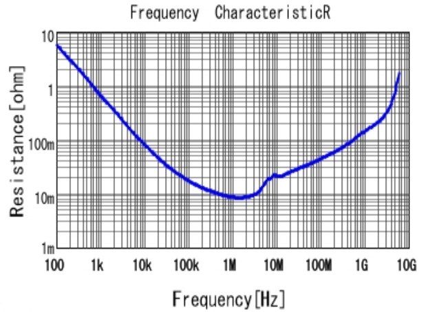
■ GRJ188C70J475KE11 R DCOV, 25degC
