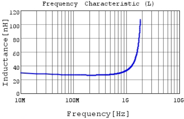
LQG18HN27NJ00 L
