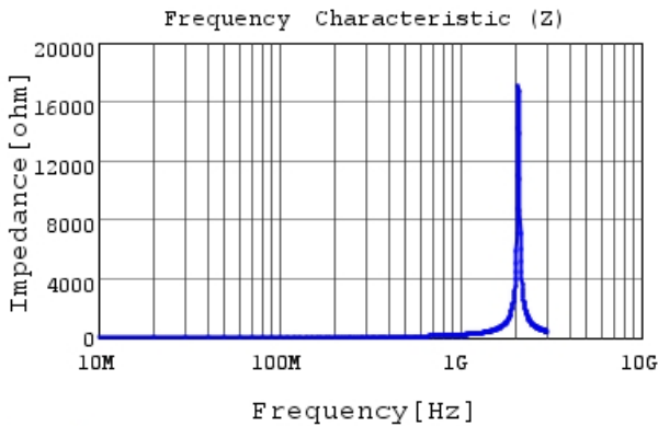
LQG18HN27NJ00 |Z|
