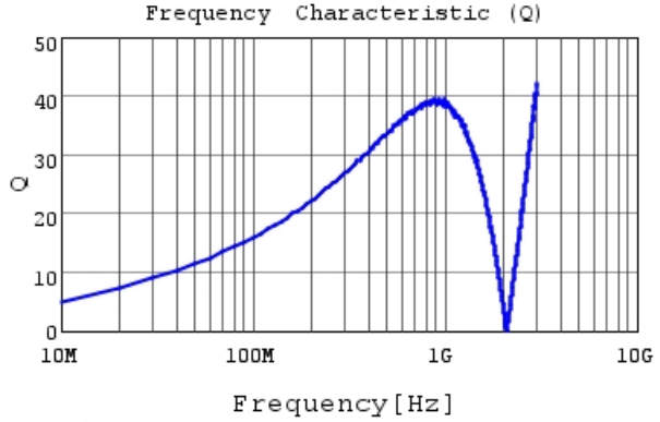
LQG18HN27NJ00 Q
