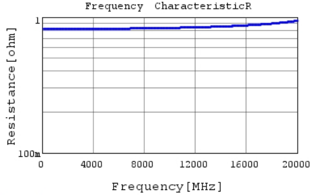
GRM0225C1ER20WA03 R DCOV, 25degC
