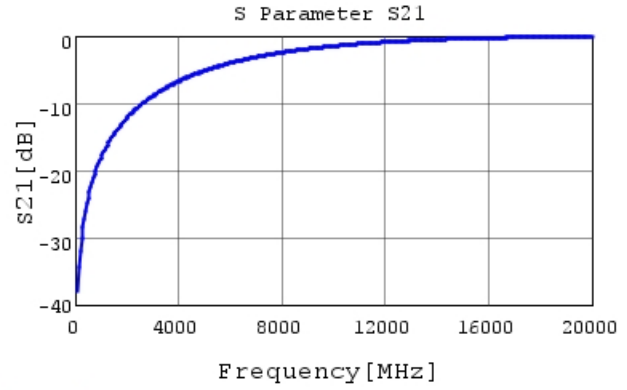
GRM0225C1ER20WA03 S21 DCOV, 25degC
