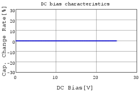
GRM0225C1ER20WA03 C-DC bias capchange, 25.0c
