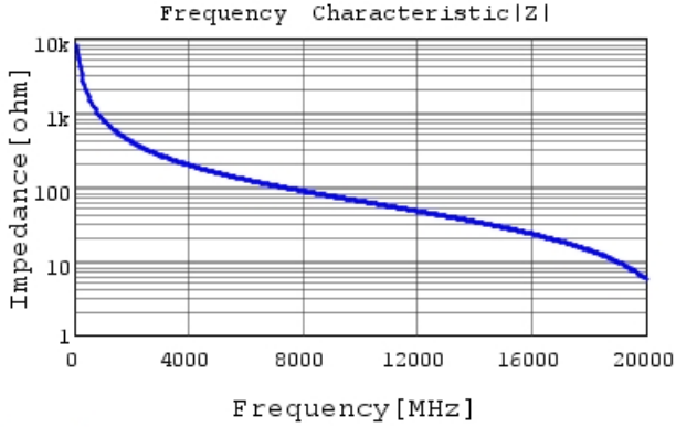
GRM0225C1ER20WA03 |Z| DCOV, 25degC
