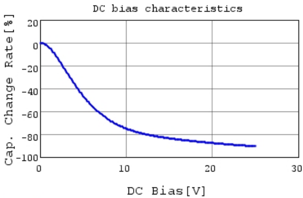
GRT033C81E104KE01 C-DC bias capchange, 25.0c
