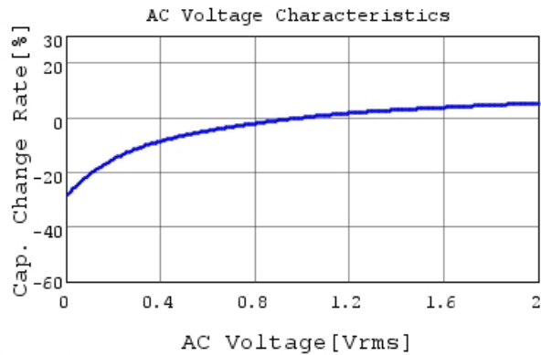
GRT033C81E104KE01 C-AC Voltage capchange, Dc
