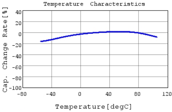
GRT033C81E104KE01 C-Temp. capchange, DC0.0V,
