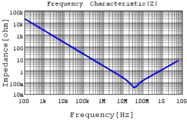
GRT033C81E104KE01 |Z| DCOV, 25degC
