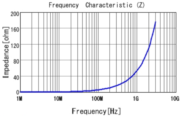
LQW03AW8N7J00 |Z|
