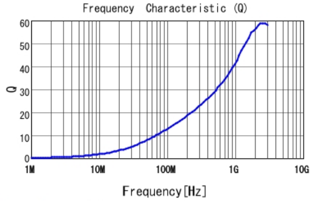
LQW03AW8N7J00 Q
