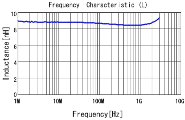
LQW03AW8N7J00 L
