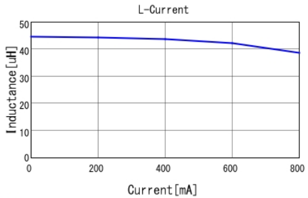
■ MDH6045C-470MB L-Current 20degC
