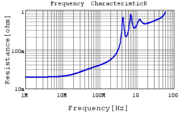
GCM1885C1H102JA16 R DCOV, 25degC
