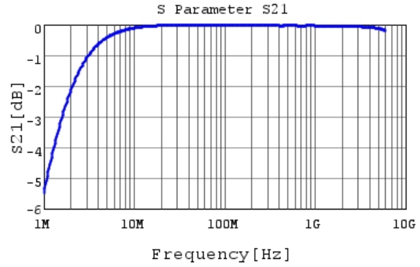
GCM1885C1H102JA16 S21 DCOV, 25degC
