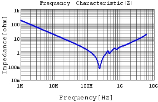
GCM1885C1H102JA16 |Z| DCOV, 25degC
