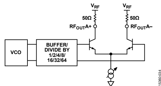
Figure 34. Output Stage
