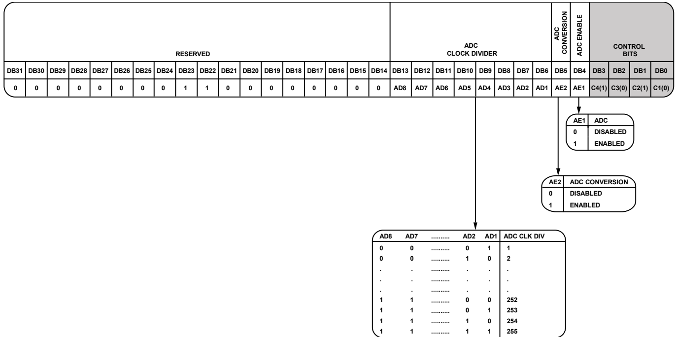
Figure 48. Register 10 Details
