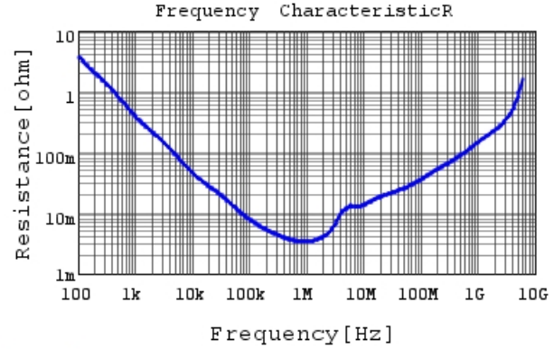
GRM188C81C106MA73 R DCOV, 25degC
