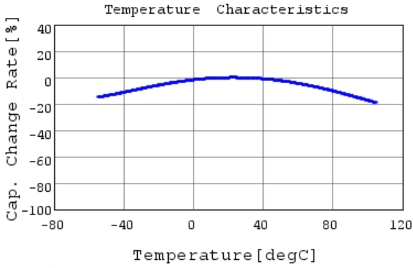
GRM188C81C106MA73 C-Temp. capchange, DC0.0V,
