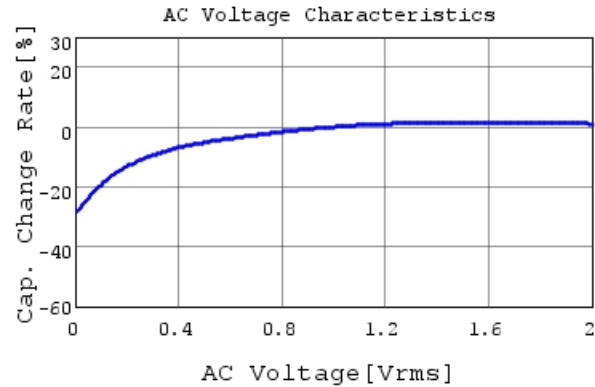
GRM188C81C106MA73 C-AC Voltage capchange, Dc
