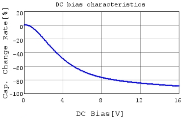
GRM188C81C106MA73 C-DC bias capchange, 25.0c
