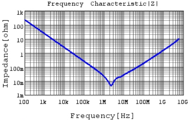
GRM188C81C106MA73 |Z| DCOV, 25degC
