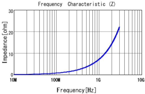
LQP03HQ1N1B02 |Z|
