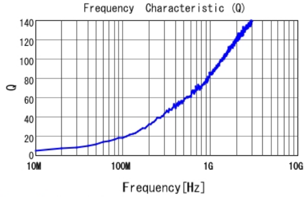
LQP03HQ1N1B02 Q
