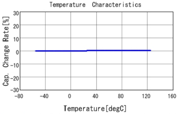
GJM1555C1H200JB01 C-Temp. capchange, DCOV, AC1Vrms
