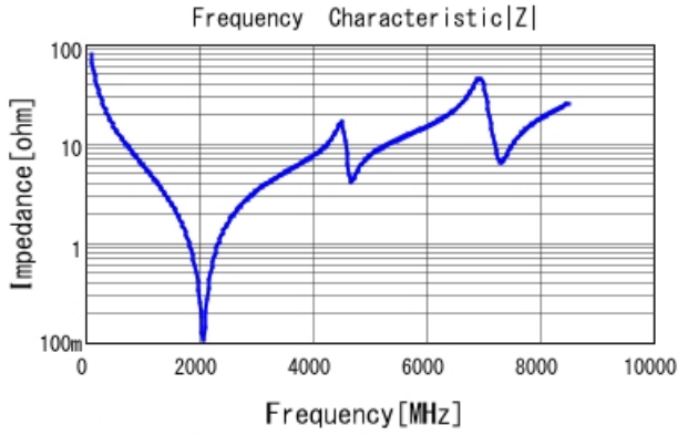
GJM1555C1H200JB01 |Z| DCOV, 25degC
