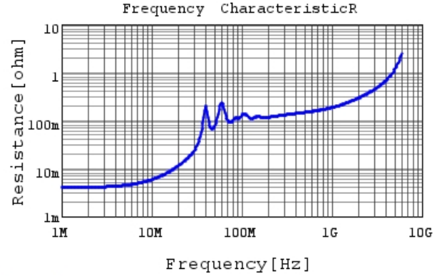
GRM31C5C1H683JA01 R DC0V, 25degC
