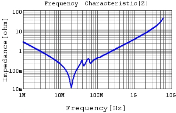
GRM31C5C1H683JA01 |Z| DC0V, 25degC
