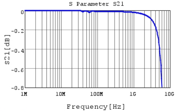
GRM31C5C1H683JA01 S21 DCOV, 25degC
