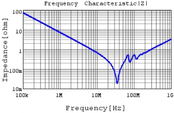
GRM31C5C2E223FWA3 |Z| DC0V, 25degC
