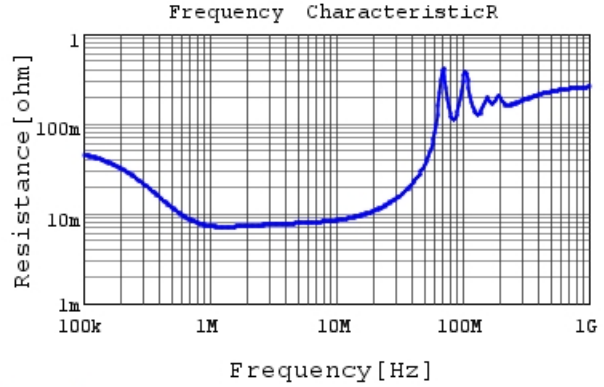
GRM31C5C2E223FWA3 R DC0V, 25degC
