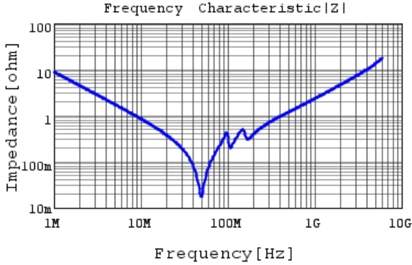
GRM21B2C1H183JA01 |Z| DCOV, 20degC
