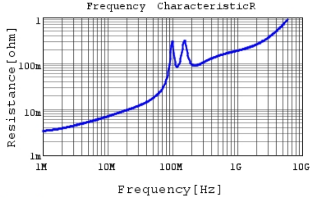
GRM21B2C1H183JA01 R DCOV, 20degC
