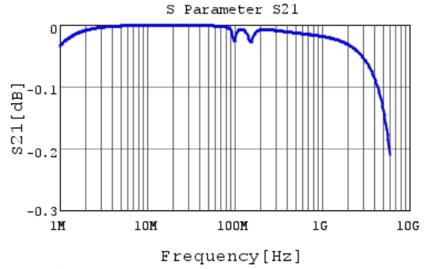
GRM21B2C1H183JA01 S21 DCOV, 20degC
