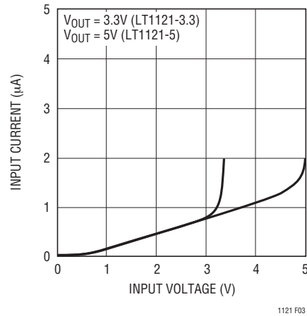
Figure 3. Input Current
