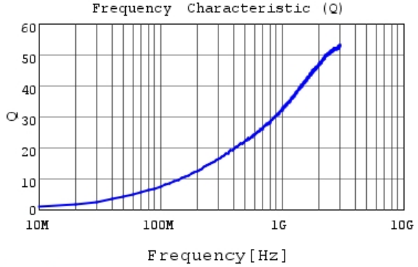
LQP15MN2N8W02 Q
