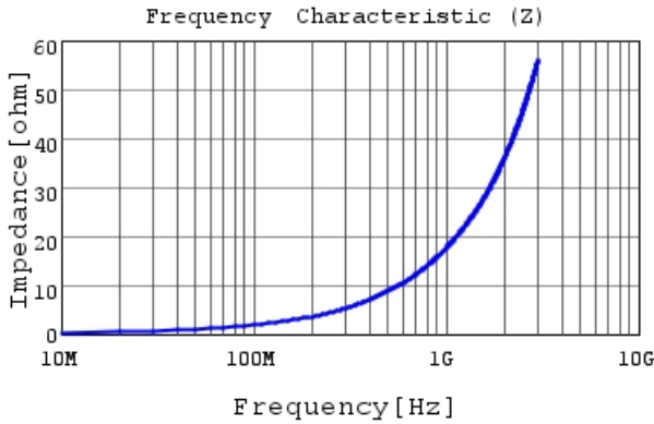
LQP15MN2N8W02 |Z|
