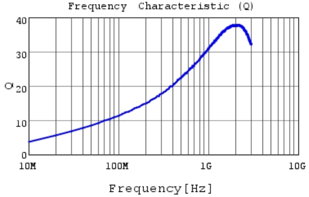
LQG15HS5N6C02 Q
