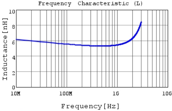
LQG15HS5N6C02 L
