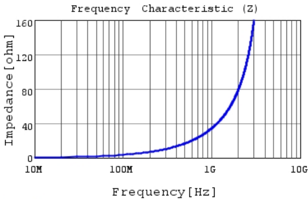
LQG15HS5N6C02 |Z|
