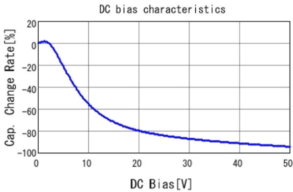
GRM219R61H225KE15 C-DC bias capchange, 25.0degC, A
