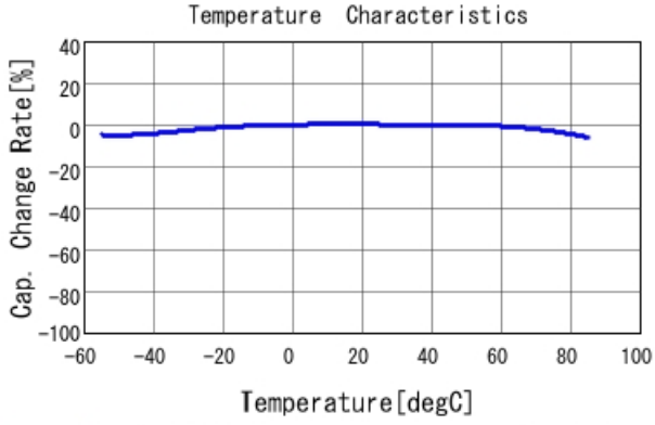
GRM219R61H225KE15 C-Temp. capchange, DC0.0V, AC1.C
