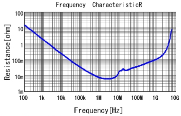
GRM219R61H225KE15 R DCOV, 25degC
