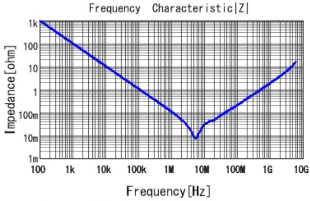
GRM219R61H225KE15 |Z| DCOV, 25degC
