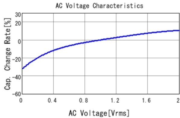
GRM219R61H225KE15 C-AC Voltage capchange, DCOV, 25
