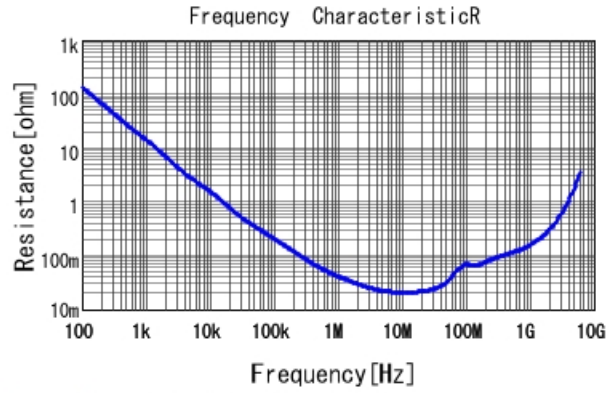
GRM155R71C683KA88 R DCOV, 25degC
