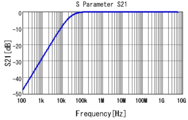
GRM155R71C683KA88 S21 DC0V, 25degC
