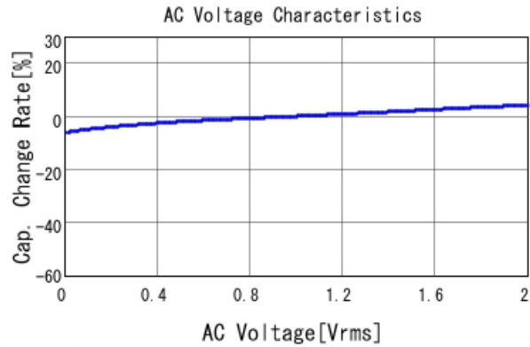
GRM155R71C683KA88 C-AC Voltage capchange, DCOV, 25
