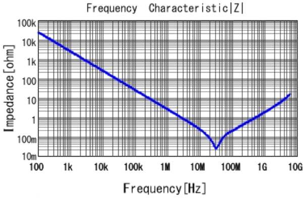
GRM155R71C683KA88 |Z| DCOV, 25degC
