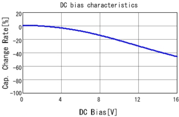
GRM155R71C683KA88 C-DC bias capchange, 25.0degC, A
