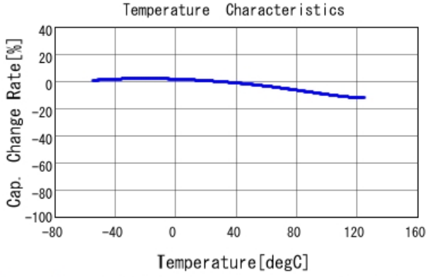
GRM155R71C683KA88 C-Temp. capchange, DC0.0V, AC1.C
