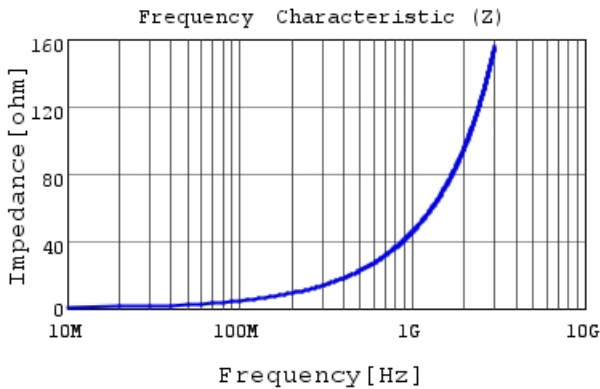
LQW15AN7N3J00 |Z|
