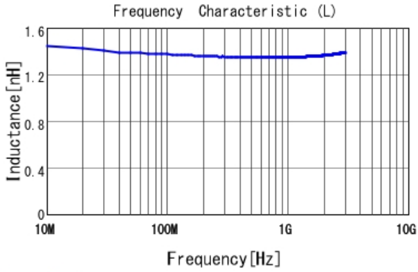
LQP03HQ1N3W02 L
