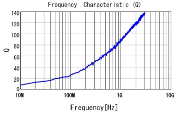
LQP03HQ1N3W02 Q
