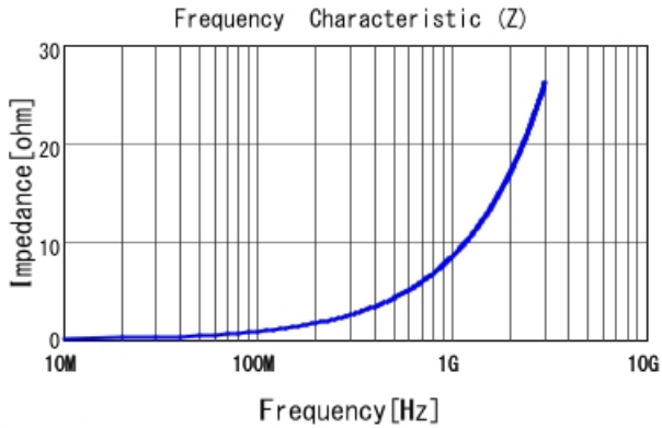
LQP03HQ1N3W02 |Z|
