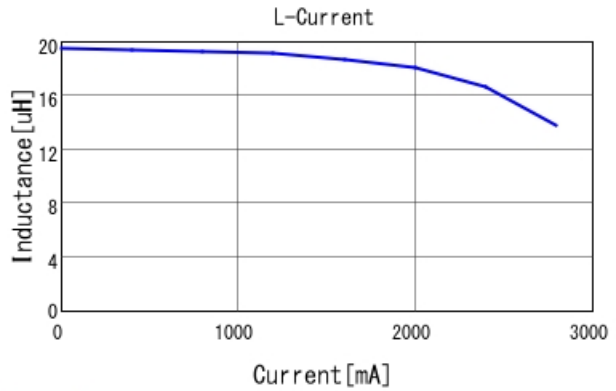
B1047AS-180M L-Current 20degC
