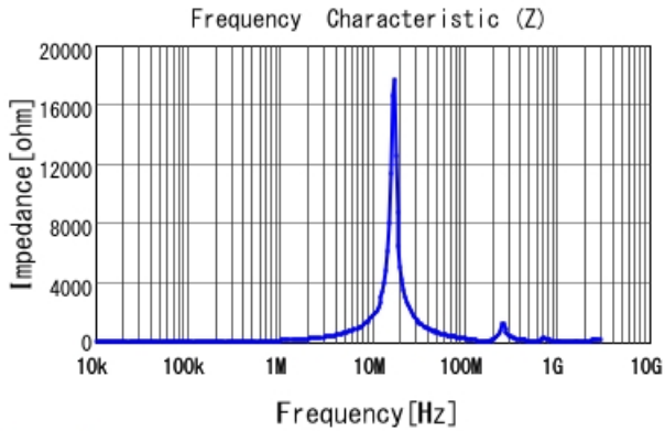
B1047AS-180M |Z|
