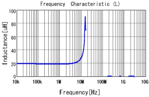
B1047AS-180M L
