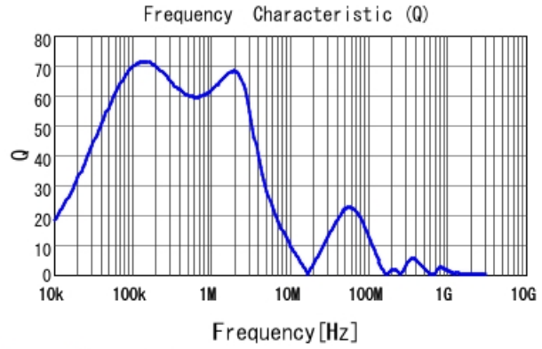
B1047AS-180M Q
