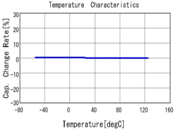
■ GRT1885C1H102JA02 C-Temp. capchange, DCOV, AC1Vrms
