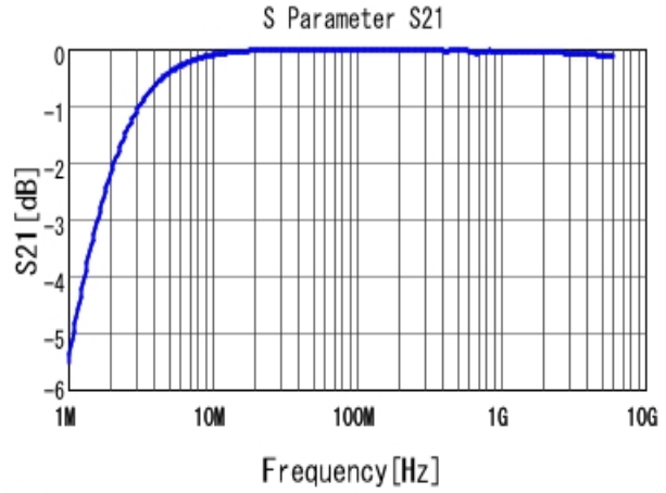
■ GRT1885C1H102JA02 S21 DCOV, 25degC
