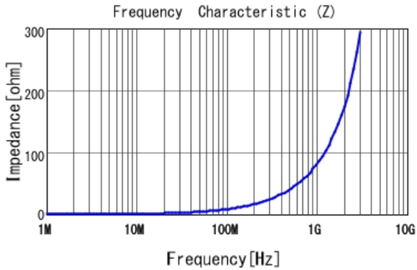
LQW03AW13NJ00 |Z|
