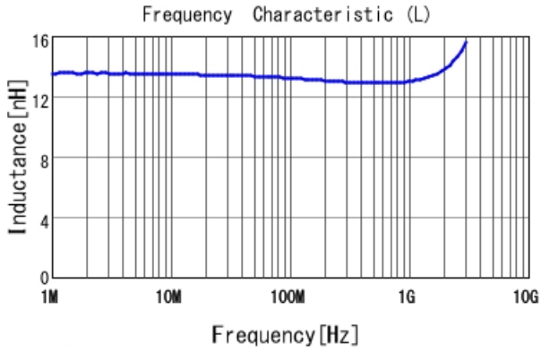
LQW03AW13NJ00 L
