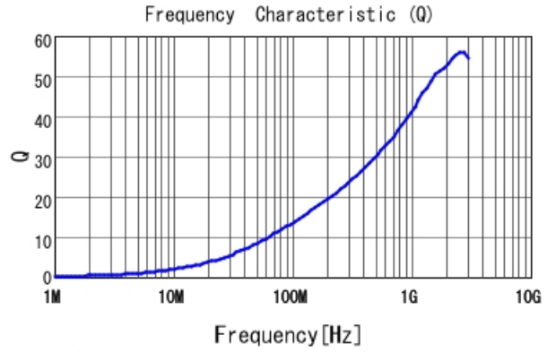
LQW03AW13NJ00 Q
