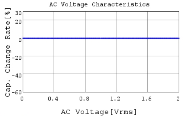
RDE5C2A820J0K1H03B C-AC Voltage capchange, I
