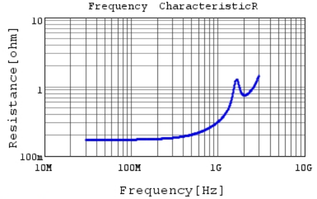
RDE5C2A820J0K1H03B R DC0V, 25degC
