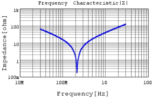
RDE5C2A820J0K1H03B |Z| DC0V, 25degC
