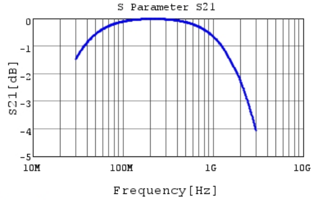
RDE5C2A820J0K1H03B S21 DCOV, 25degC
