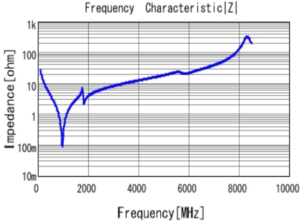
■ GQM1885C1H560JB01 |Z| DC0V, 25degC
