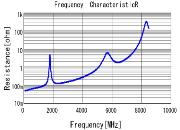
■ GQM1885C1H560JB01 R DC0V, 25degC
