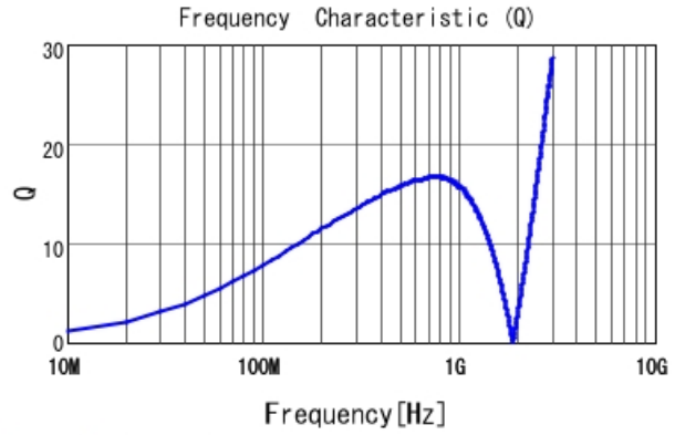
LQP03TN47NJZ2 Q
