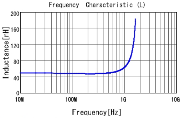
LQP03TN47NJZ2 L
