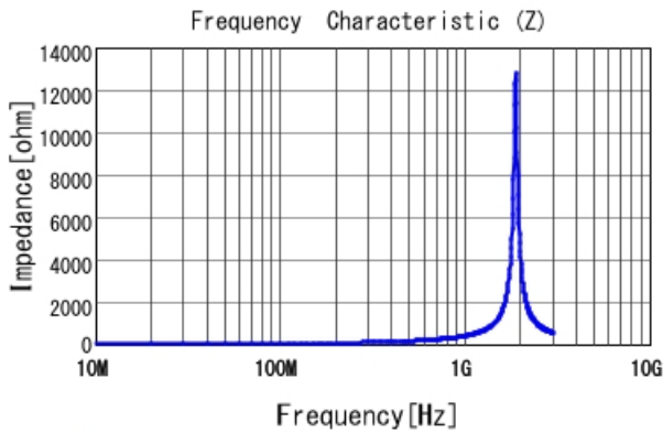
LQP03TN47NJZ2 |Z|
