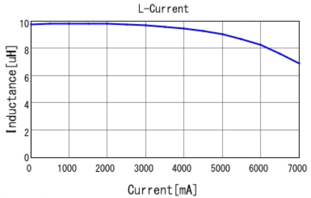
#B966AS-100M=P3 L-Current 20degC
