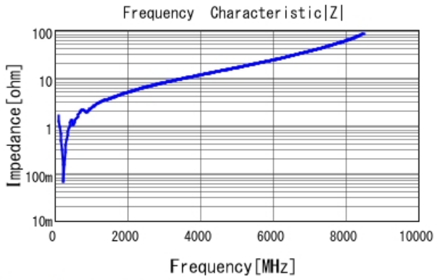
GRM1885C1H821JA01 |Z| DCOV, 25degC
