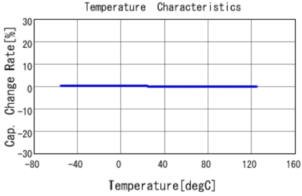
GRM1885C1H821JA01 C-Temp. capchange, DCOV, AC1Vrms
