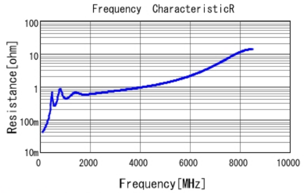
GRM1885C1H821JA01 R DCOV, 25degC
