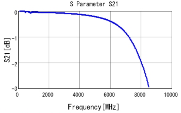
GRM1885C1H821JA01 S21 DCOV, 25degC
