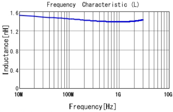
LQP03TN1N4BZ2 L
