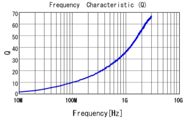
LQP03TN1N4BZ2 Q
