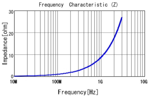
LQP03TN1N4BZ2 |Z|
