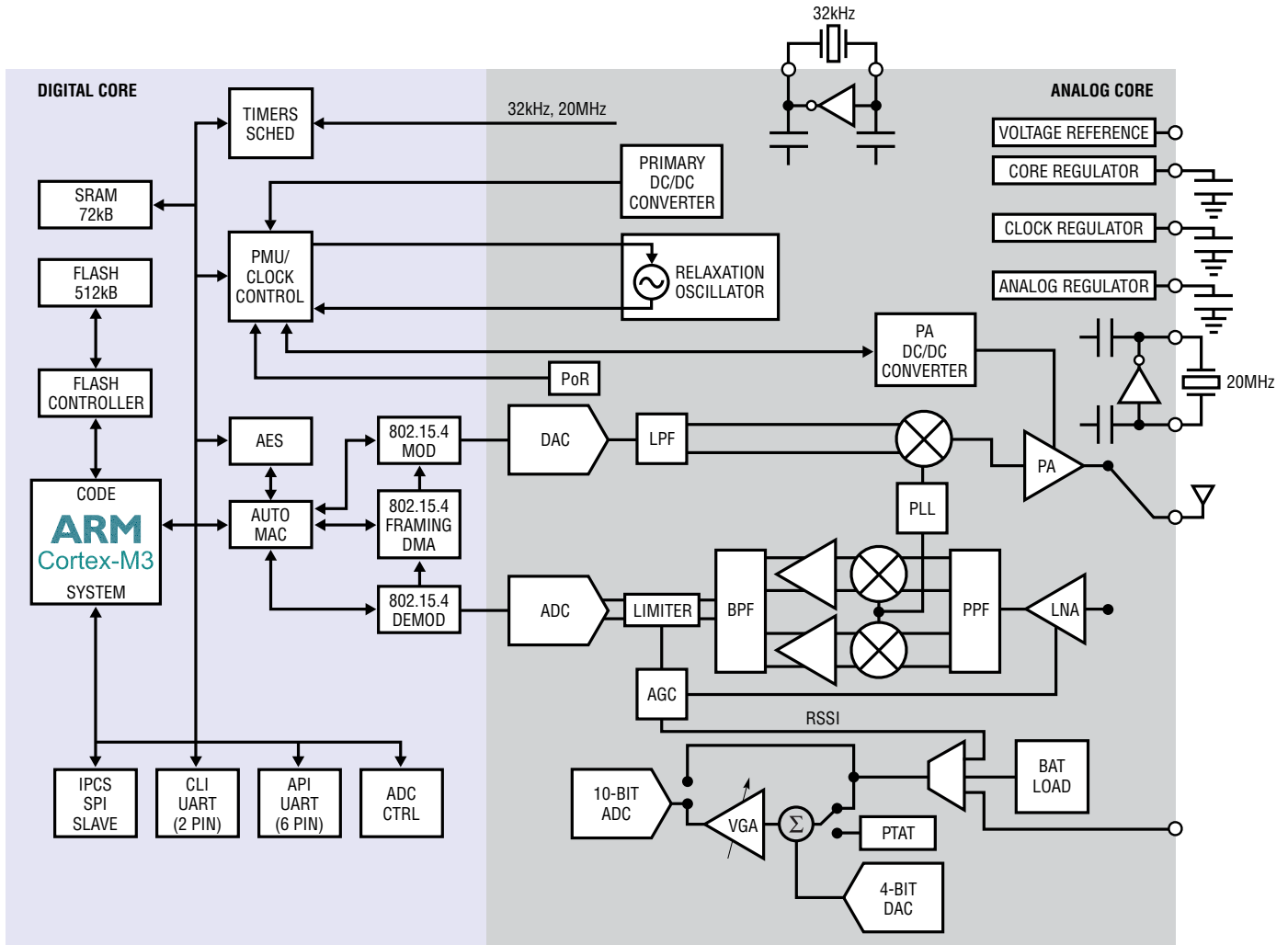
Figure 9 . Eterna Block Diagram
