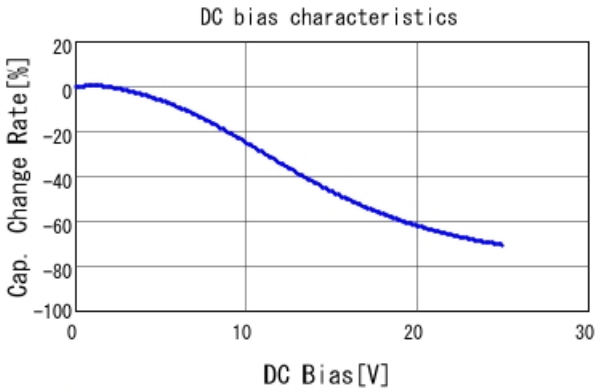
GRM155R61E104KA87 C-DC bias capchange, 25.0degC, A
