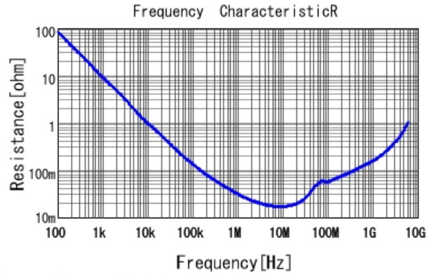
GRM155R61E104KA87 R DCOV, 25degC
