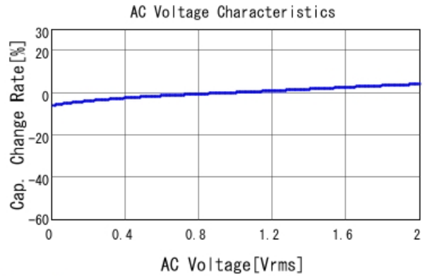
GRM155R61E104KA87 C-AC Voltage capchange, DCOV, 25
