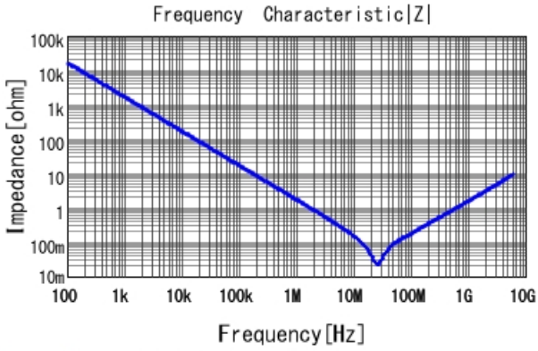
GRM155R61E104KA87 |Z| DCOV, 25degC
