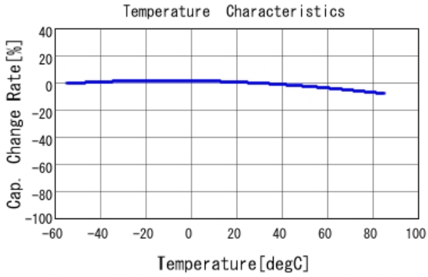
GRM155R61E104KA87 C-Temp. capchange, DC0.0V, AC1.C
