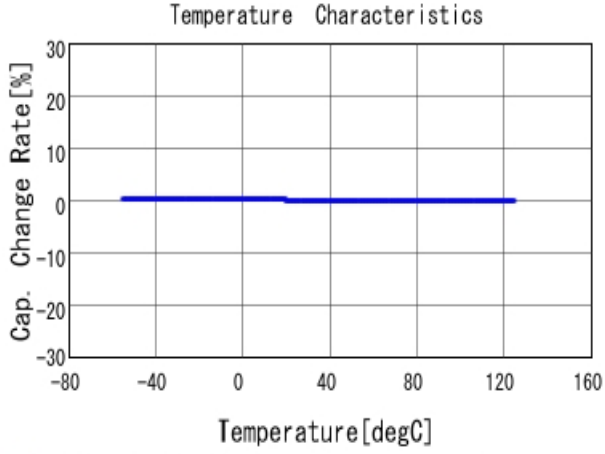
■ GRM1552C1H821JA01 C-Temp. capchange, DCOV, AC1Vrms
