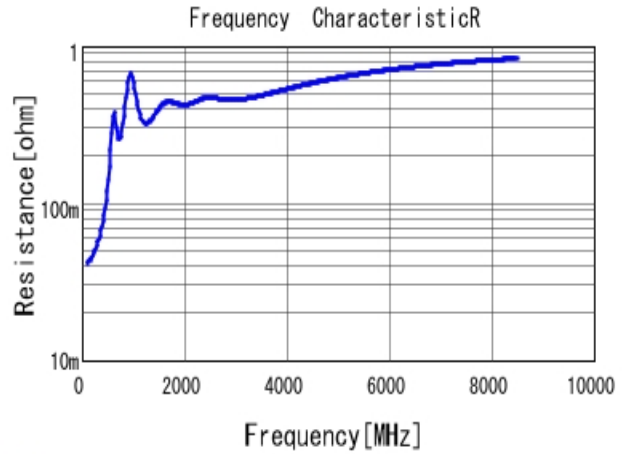
■ GRM1552C1H821JA01 R DCOV, 20degC
