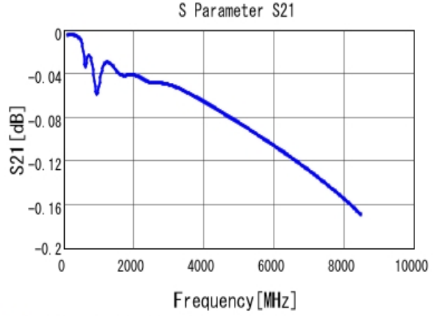
■ GRM1552C1H821JA01 S21 DCOV, 20degC
