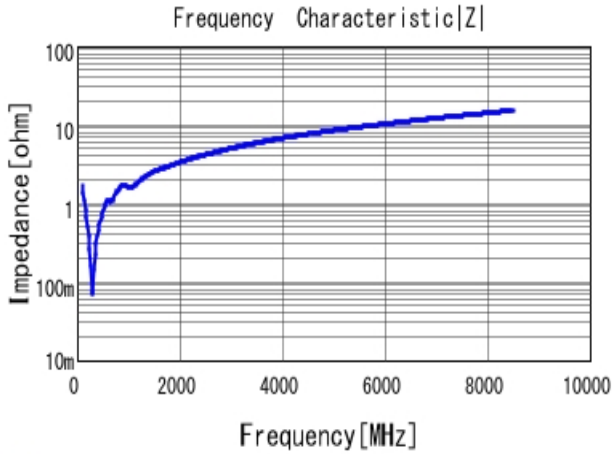
■ GRM1552C1H821JA01 |Z| DCOV, 20degC
