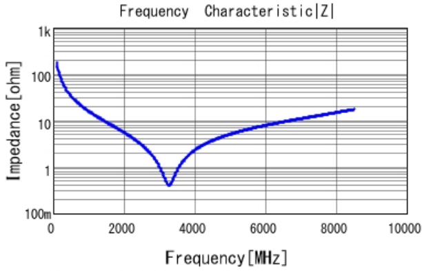
GRM0335C1H9R1BA01 |Z| DCOV, 25degC
