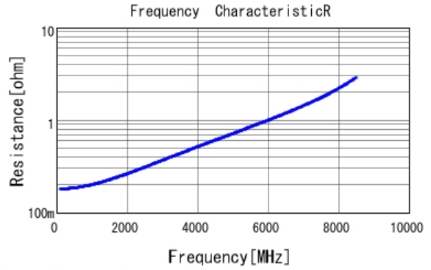
GRM0335C1H9R1BA01 R DCOV, 25degC
