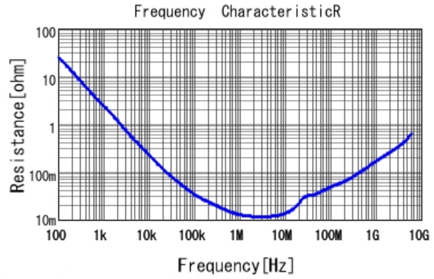
GRM155R61A474ME15 R DCOV, 25degC
