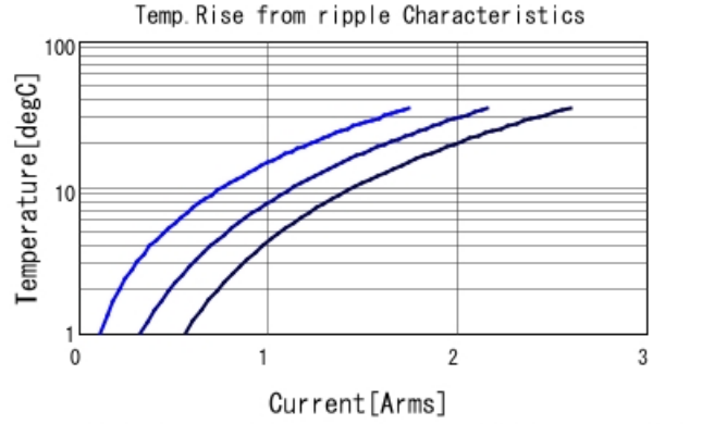
GRM155R61A474ME15 Temp. rise — 100kHz — 500
