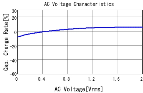
GRM155R61A474ME15 C-AC Voltage capchange, DCOV, 25
