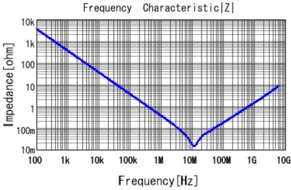
GRM155R61A474ME15 |Z| DCOV, 25degC
