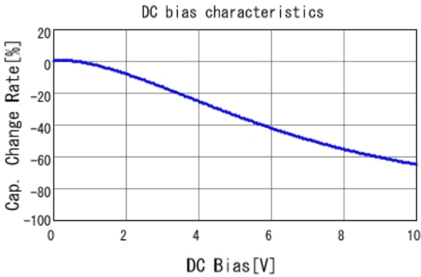
GRM155R61A474ME15 C-DC bias capchange, 25.0degC, A
