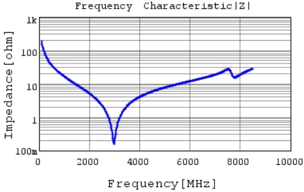
GCQ1555C1H8R6BB01 |Z| DC0V, 25degC
