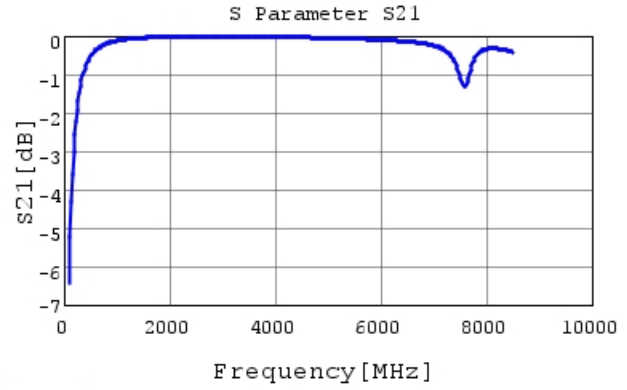
GCQ1555C1H8R6BB01 S21 DCOV, 25degC
