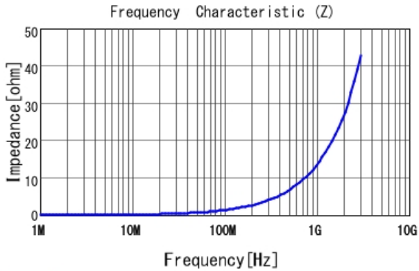
LQW15AN2N2C80 |Z|
