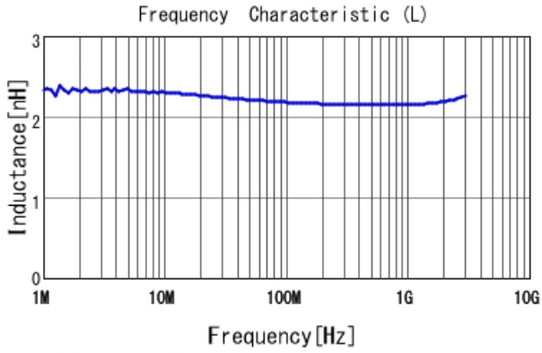
LQW15AN2N2C80 L
