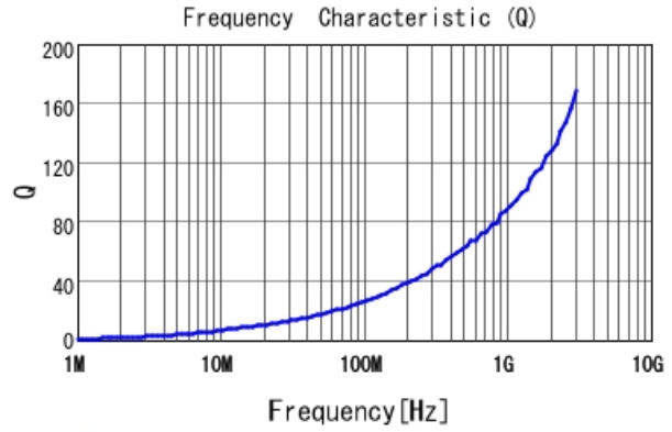
LQW15AN2N2C80 Q
