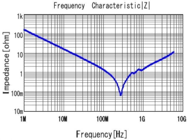
■ GRM1552C1E102JA01 |Z| DCOV, 20degC
