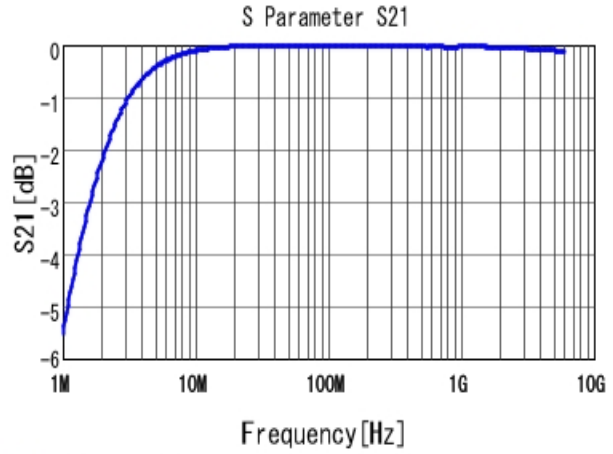
■ GRM1552C1E102JA01 S21 DCOV, 20degC
