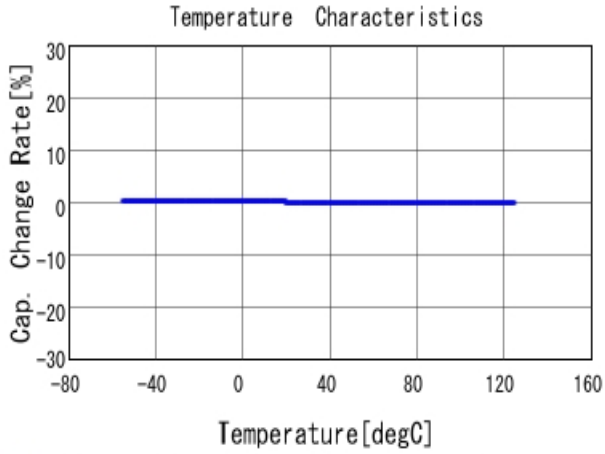
■ GRM1552C1E102JA01 C-Temp. capchange, DCOV, AC1Vrms
