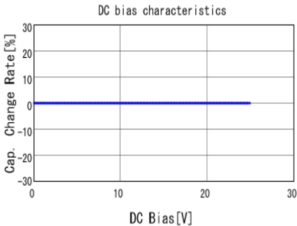
■ GRM1552C1E102JA01 C-DC bias capchange, 20.0degC, AC1V
