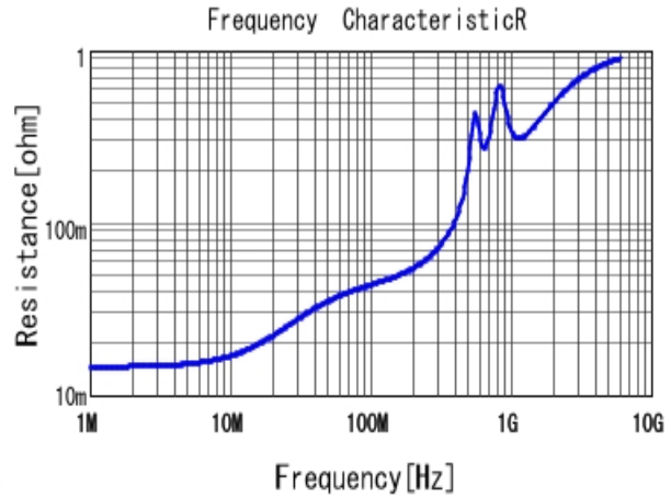
■ GRM1552C1E102JA01 R DCOV, 20degC
