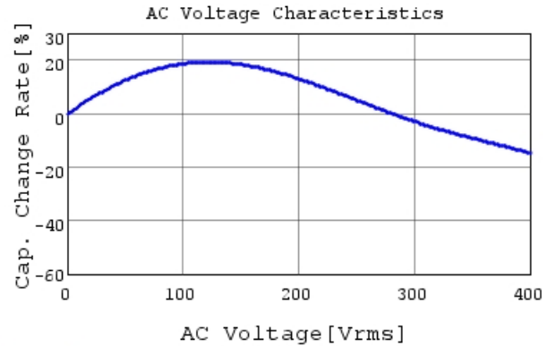
RDER73A103K2K1H03B C-AC Voltage capchange, I
