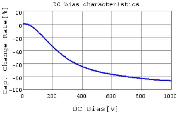
RDER73A103K2K1H03B C-DC bias capchange, 25.0
