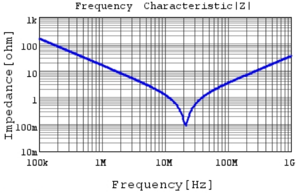
RDER73A103K2K1H03B |Z| DCOV, 25degC
