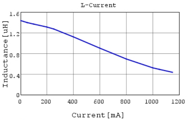
LQM21PN1R5MCH L-Current 20degC
