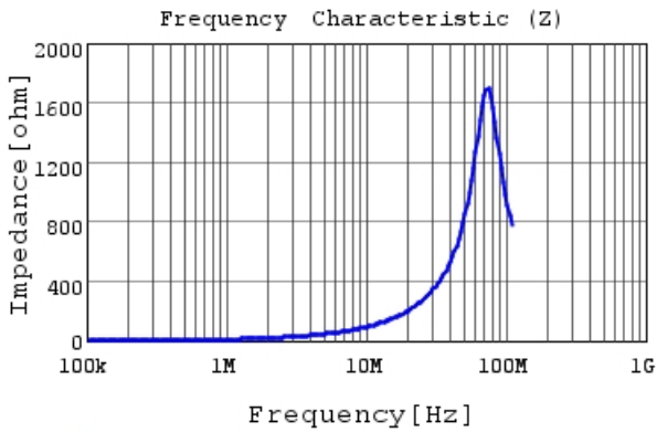
LQM21PN1R5MCH |Z|
