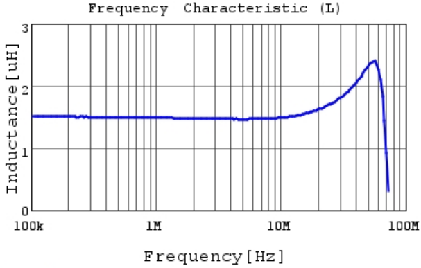
LQM21PN1R5MCH L
