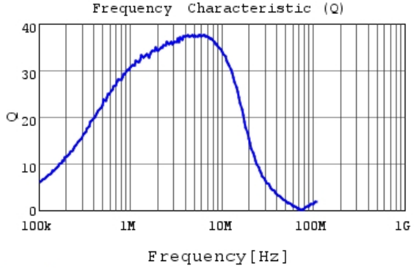
LQM21PN1R5MCH Q
