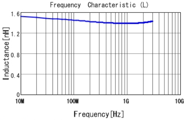
LQP03TN1N4B02 L
