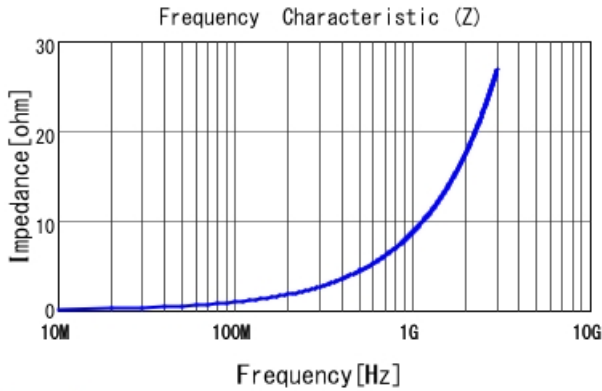
LQP03TN1N4B02 |Z|
