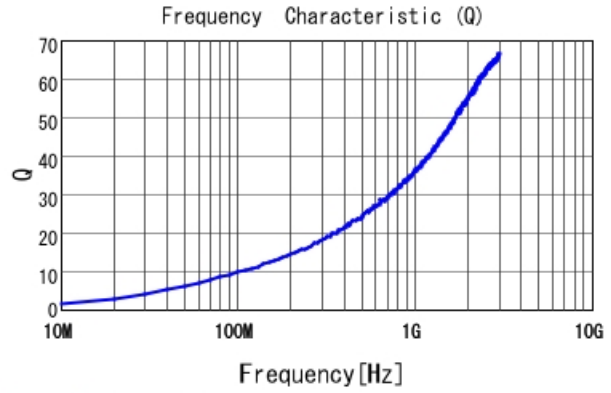
LQP03TN1N4B02 Q
