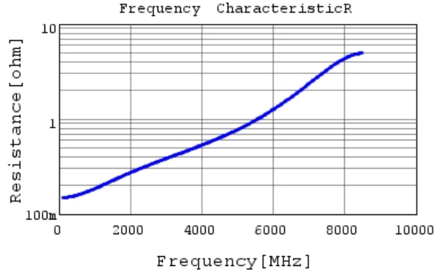
GCM0335C1E220JA16 R DC0V, 25degC
