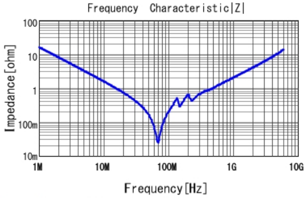
GRM2192C1H103JA01 |Z| DCOV, 20degC
