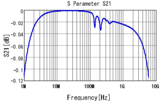
GRM2192C1H103JA01 S21 DCOV, 20degC
