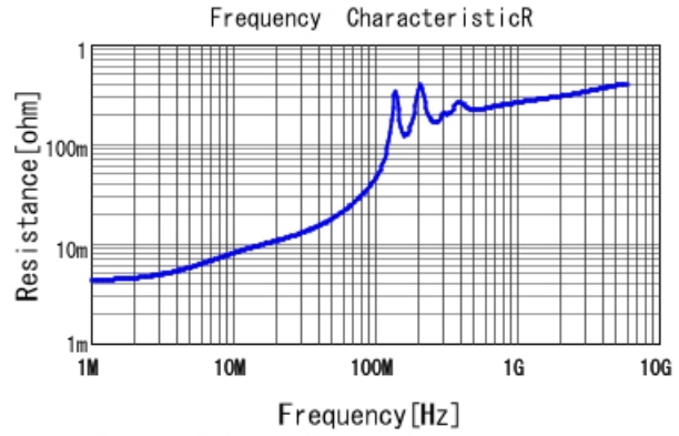
GRM2192C1H103JA01 R DCOV, 20degC
