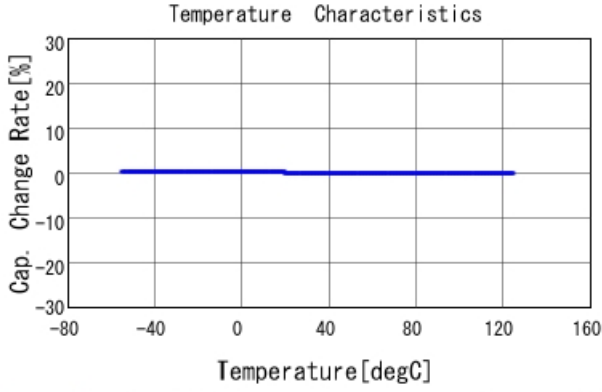
GRM2192C1H103JA01 C-Temp. capchange, DCOV, AC1Vrms
